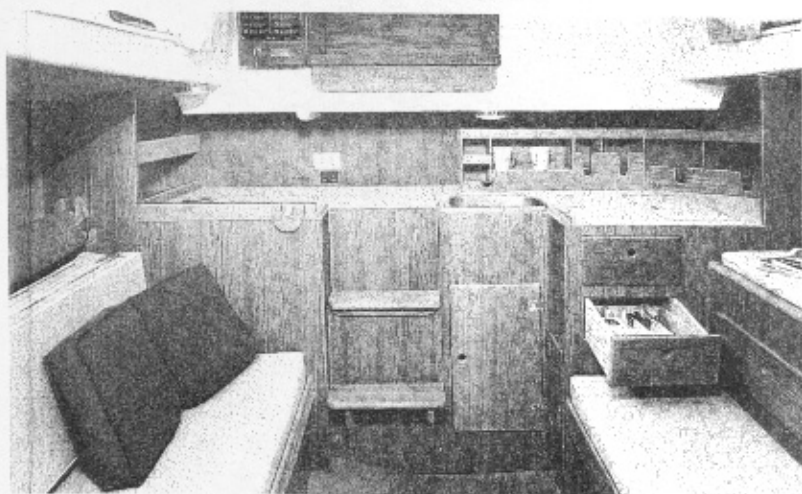
VANGUARD CABIN PLAN
